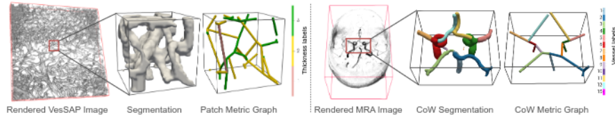
Fig. 2. Two real-world vessel datasets. Left. An example from VesSAP and the capillary level vessel graph patch. Right. The extracted metric graph for the blood vessel in CoW. (Best viewed when zoomed in)
