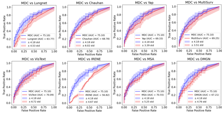
Fig. 2. Mean ROC curves of 5-fold cross validation on all the 8 compared methods with mean AUC values \pm standard deviation (std) on the EF prognosis.
