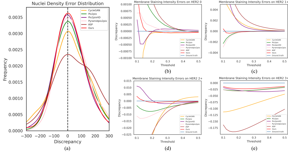
Fig. 3. The error analysis of task-specific domain knowledge. (a) Nuclei density error distribution of all methods. (b)-(e) Membrane staining intensity errors grouped by HER2 scores. The representation of HER2 scores here is the same as Fig. 2.
