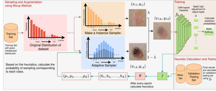
Fig. 1. Our Proposed Framework
