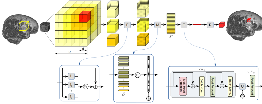
Fig. 1. Proposed method. F : Frequency encoding block, where f_1 - f_n denote different frequency encodings and P_1 is positional encoding. M : Positional encoding and masking, where P_2 is positional encoding and B denotes a Bernoulli random process used to mask the sequence. T : Vision transformer block. U : Unmasking. R : Reshaping.
