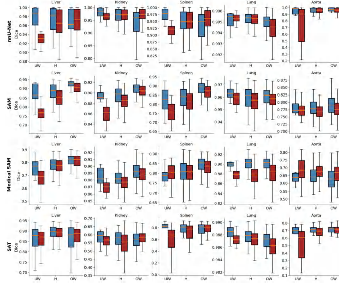
Fig. 2. Segmentation performance (means and standard deviations) for subject groups specified by combinations of gender and BMI attributes. Blue box: male. Red box: female. UW: Underweight, H: Healthy, OW: Overweight.
