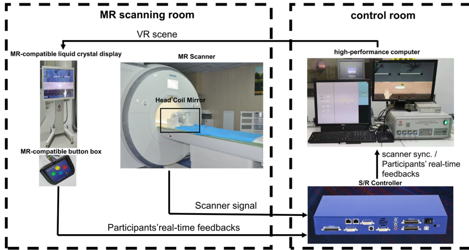
Fig. 1. An overview of the MR.VRA system's hardware logic. The arrows indicate the transmission direction of signal and data flows.
