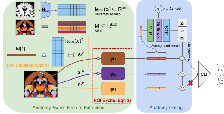
Fig. 1: Overview of AAGN. An anatomy-aware squeeze-and-excite operation extracts features from the CNN feature map for each ROI. The ROI feature embeddings are concatenated to form a context vector representing the overall brain state. The Anatomy Gating Network uses this context vector to dynamically determine which regions are relevant. A permutation-invariant classifier is trained on the selected regions and provides feedback on which ROIs to select.
