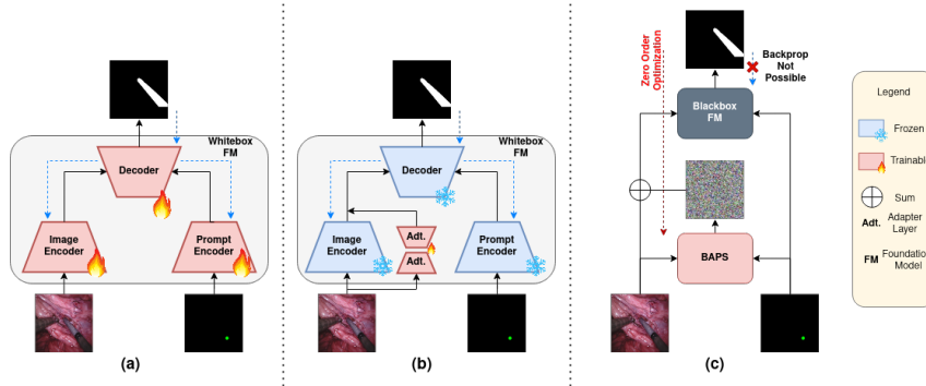
Fig. 1: Comparison of our method (c) against full finetuning of a Foundation Model (FM), (a) and common adaptation techniques (b).
