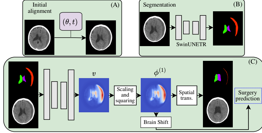
Fig. 2. Overview of our process. Images are aligned to a sagittal plane (A) and automatically segmented (B). The CT scan and segmentations are used as input to a deep diffeomorphic registration model (C). Deformation fields provided by this model are used to distinguish between patients requiring surgery by various biomarkers.
