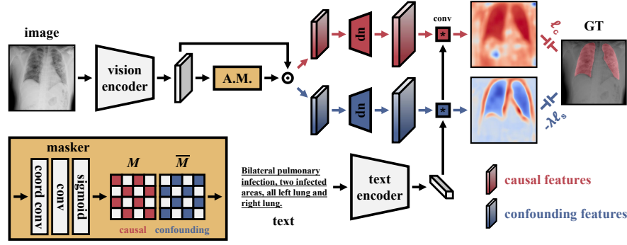
Fig. 1. Overview of the proposed CausalCLIPSeg model.
