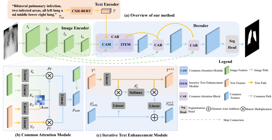
Fig. 2. Overview of our proposed method and detail of the modules. Our model mainly consists of an image encoder, a text encoder and a multi-modal decoder. The decoder contains three Common Attention Blocks (CAB) to fuse and decode the multimodal features layer-by-layer, while each CAB contains a Common Attention Module (CAM) and Iterative Text Enhancement Module (ITEM).
