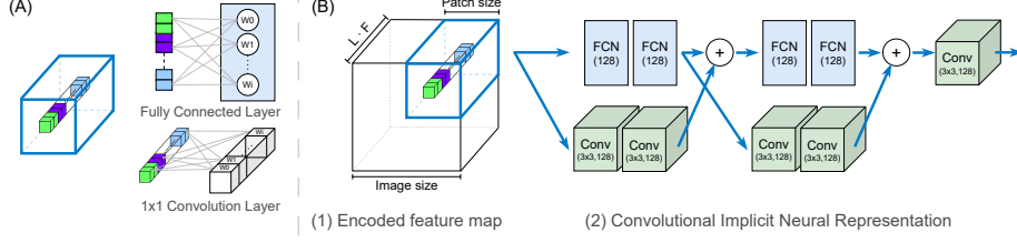
Fig. 1. (A) Fully Connected and Convolutional Layers: These layers are interchangeable if the convolutional layer has a kernel size of 1 \times 1 . The kernel values correspond to the weights in the fully connected layer. (B) Our Convolutional Implicit Neural Representation (CINR) Model: The collection of feature vectors from all target pixels is represented as a 3D tensor. This tensor is divided into multiple patches, with each patch processed by the model. The processing can occur in one of two ways: 1) treating all feature vectors within a patch as a batch, or 2) processing the 3D patch directly. In the model, each rectangle box represents a fully connected layer, and each cube box represents a convolutional layer.
