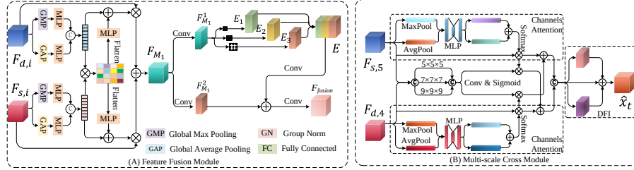
Fig. 2. (A) FFM. F_{d,i} is the features of i stage in the encoder of the DU; (B) MCM. This module is processed with a set of convolutional blocks with kernels of different sizes to capture multi-scale features. F_{s,5} is the feature obtained through graph reasoning.
