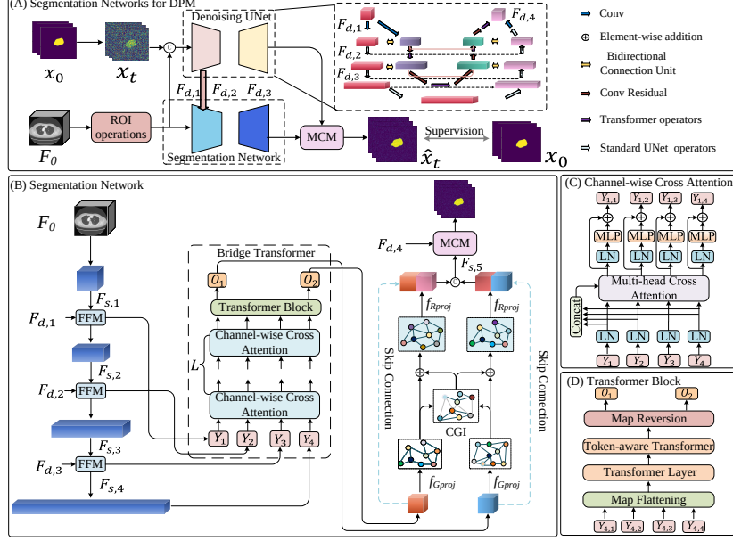
Fig. 1. Overview of the Diff-UNet proposed in this study. F_{s,i} is the feature of i stage of the encoder in the segmentation network. The bidirectional connection units use convolutional layers to refine deep features and interactively connect the two branches.
