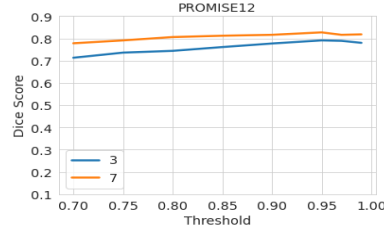
Fig. 3: Ablation on confidence threshold values for PROMISE12.
