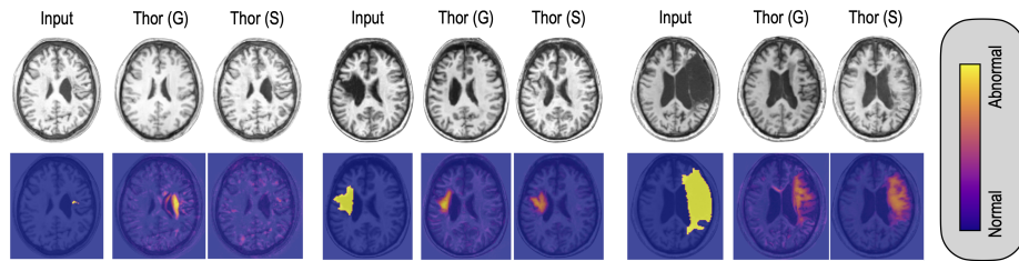
Fig. 3: Anomaly detection in brain MRI scans processed by THOR using Gaussian (G) and Simplex (S) noise. From left to right, the lesions increase in size, with the smallest representing a challenging case.
