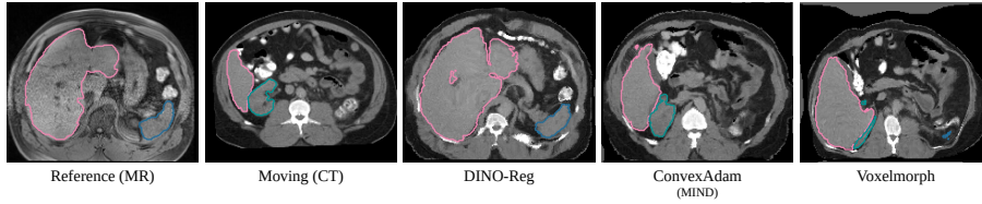
Fig. 2. Qualitative registration result from abdomen MR-CT dataset. All images are placed on the same slice as the reference image.
