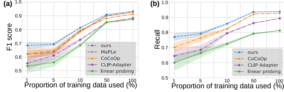
Fig. 3. Data efficiency on (a) kidney cancer in PanNuke and (b) COVID in COVID-x.
