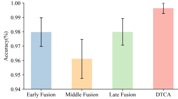
Fig. 6. Comparison results with different fusion methods based on SEED-IV
