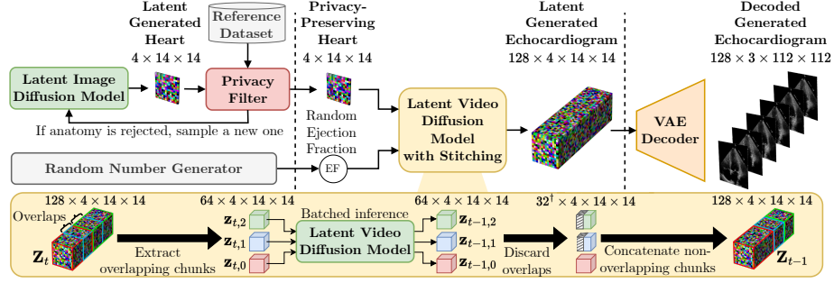
Fig. 1. Our inference video generation pipeline, consisting of a latent image diffusion model with a privacy filter, a latent video diffusion model with video stitching and a VAE decoder. All dimensions are given in (time \times ) channels \times height \times width. \dagger In the video stitching method (yellow block), the first half of \mathbf{z}_{t-1,0} is not discarded.
