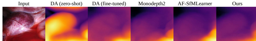
Fig. 3. Qualitative depth comparison on the SCARED dataset.
