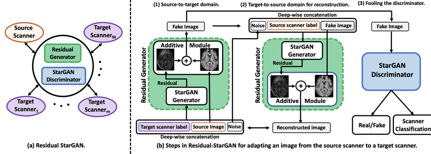
Fig. 2: Illustration of Residual StarGAN
