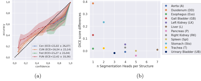
Fig. 4: Calibration of the different methods in terms of Expected Calibration Error (a) and performance gain of FUNAvg in comparison to vanilla averaging the different logits from the federated training segmentation heads (b).
