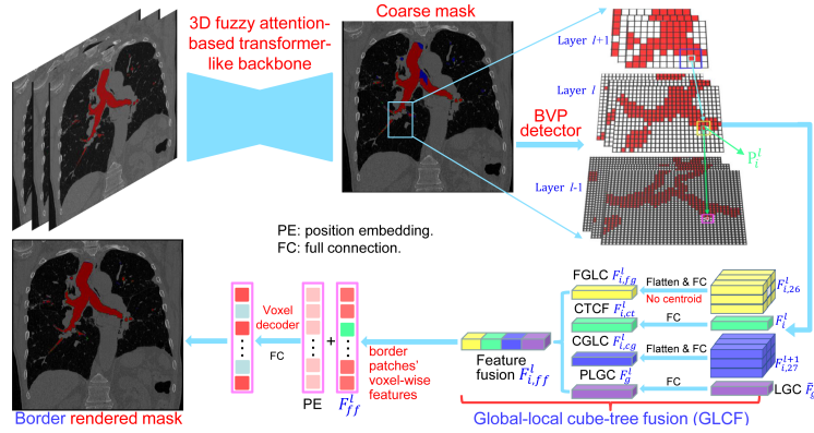
Fig. 2. The overview of our method FABR. FGLC: fine grain local context; CTCF: cube-tree centroid feature; CGLC: coarse grain local context; PLGC: projected learnable global context. BVP detector is shown in Fig. 1. Noting the matched relationship between top-right boxes’ and bottom-right bars’ colors.
