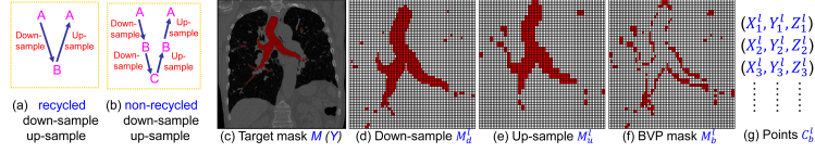
Fig. 1. The elaboration of B order V ulnerable P oints (BVP) caused by recycled down-sample and up-sample in the encoder-decoder backbone. Downsampling (c) gets (d), upsampling (d) gets (e), then (f) is the absolute difference of (c) & (e). In the test phase, (c) is binarized coarse prediction.
