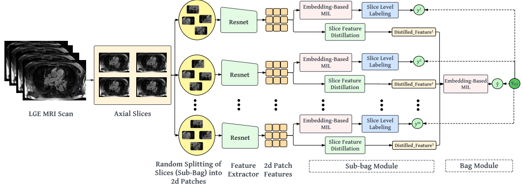
Fig. 1: Overview of our proposed model. For illustrative purposes, we select M axial slices (with 4 depicted as an example) at random from an LGE MRI scan, treating each slice as an individual sub-bag. We then extract random cropped patches from each of these slices. These sub-bags are initially processed by the sub-bag module. Subsequently, the output from sub-bag module is used to generate feature vectors, which are then input into the bag module. It is important to note that the ground truth label for the bags remains consistent across both sub-bag module and bag module during the training phase.
