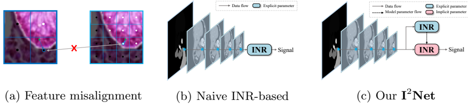
Fig. 1. a) An example of context mismatch occurring at the input coordinate ( \star ) in INR. b) Naive INR-based decoders representing segmentation maps with explicit/static parameters. c) Our I^2 Net representing maps with implicit/dynamic parameters, which is further represented with an explicit/static INR.
