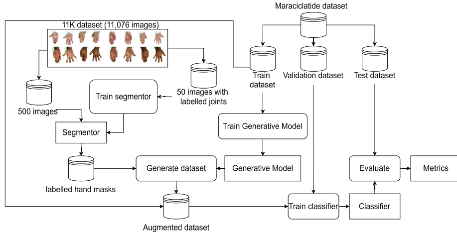
Fig. 4. Overview of the augmentation method using the 11k publicly available dataset for a single cross fold. The ^{99m}\text{Tc} maraciclatiside dataset is split into a 60% train, 20% validation, 20% test; the validation and test datasets were used in the model training and testing without modification. The diffusion model was trained on the ^{99m}\text{Tc} maraciclatiside images in the train dataset with clinician defined labels. The images from the 11k dataset were labelled with a segmentor network that labels all the joint regions in the hands; the hand masks were generated through a preprocessing algorithm. These labelled 11k images with joints are then randomly sampled to generate ^{99m}\text{Tc} maraciclatiside synthetic version. The augmented train dataset is comprised of the ^{99m}\text{Tc} maraciclatiside train dataset as well as the 11k augmented images. The trained classifier was then evaluated on the test dataset.
