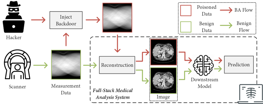
Fig. 1. The diagnosis pipelines of the proposed method with benign data and poisoned data.
