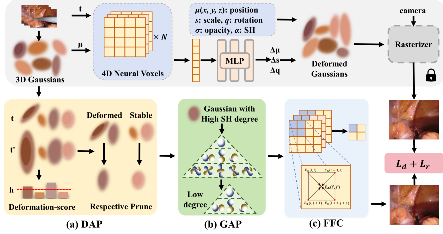
Fig. 1. LGS Overview consists of (a) Deformation-Aware Pruning, (b) Gaussian-Attribute Pruning, (c) Feature Field Condensation, and distillation for optimization.
