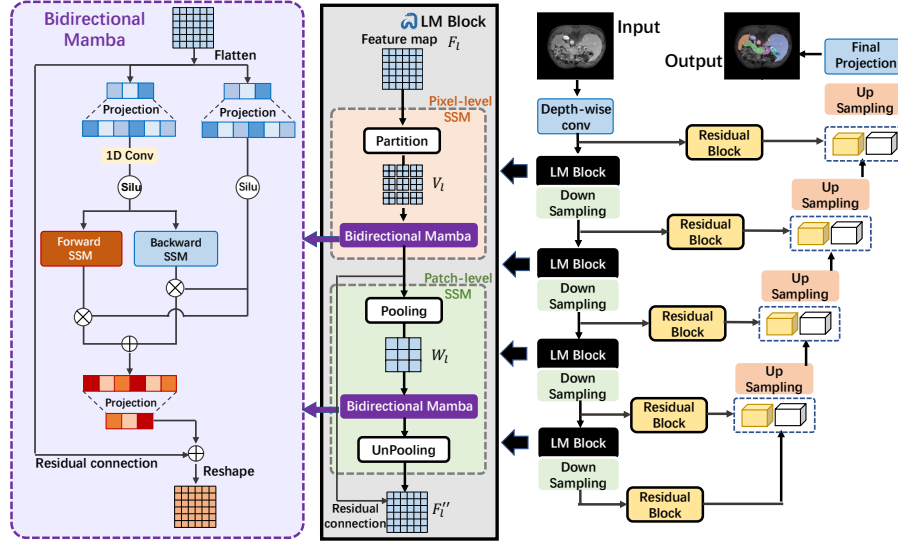
Fig. 1. An overview of our proposed LKM-UNet.
