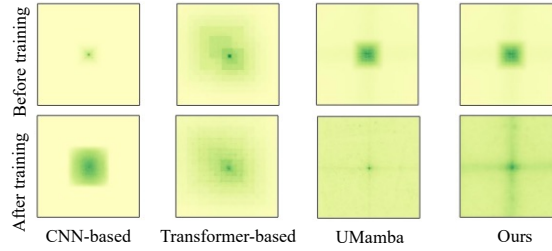
Fig. 3. Effective receptive field visualization among CNN, Transformer, U-Mamba and our proposed LKM-UNet.
