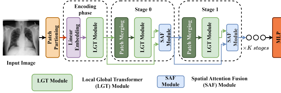
Fig. 1. Architecture of the proposed Med-Former.
