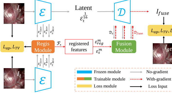
Fig. 1. The designed architecture based on KL-Reg VQ-GAN.
