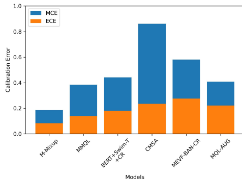
Fig. 3. The calibration error of different models.
