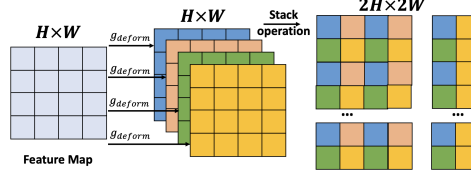
Fig. 3. Implementation of Region-aware Implicit Function. To learn flexible regions, an offset convolution layer ( g_{\text{deform}} ) is used to learn the offset, taking the feature value at x_q in the continuous feature map M as input.
