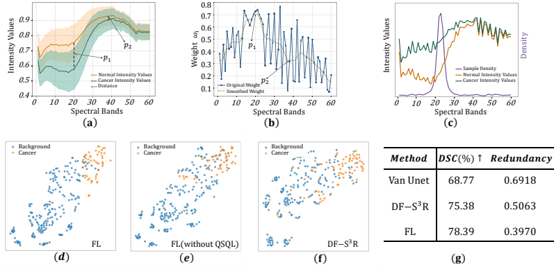
Fig. 4. (a): Spectral intensity in MDC dataset. (b): Spectral focal coefficients distribution. (c): Sampled points distribution in the Indicative Spatiospectral Transformer module of one image in MDC dataset and its corresponding spectral intensity plot. (d)-(f): t-SNE visualization of the first layer features from the Decoder across different methods. (g): Feature redundancy in MDC dataset.
