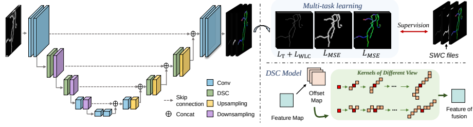
Fig. 1. The framework of NeuroLink. The green blocks in the second and third layers of the network correspond to the DSC module. The network produces outputs with five channels, comprising probability map, distance transformation map, and three components of direction vector.
