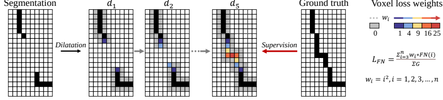
Fig. 2. A toy example of l_{FN} . We identify false negative voxels sequentially through dilation and apply weighted penalties.
