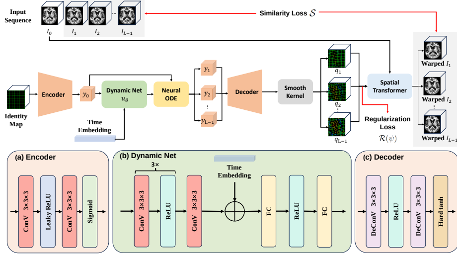
Fig. 1. Overview of our proposed NODER framework.
