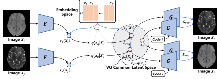
Fig. 1. Overview of the proposed VQ-Seq2Seq framework.
