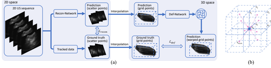
Fig. 1. (a) Overview of the proposed method with rigid transformation and nonrigid deformation prediction. (b) Contributions from support data to query data.
