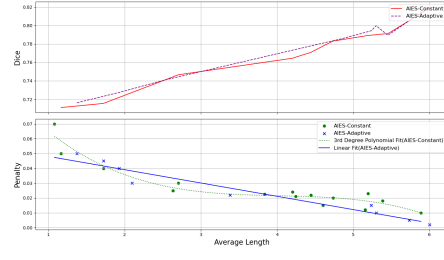
Fig. 2: The top plot shows Average length vs. Dice coefficient (LOWESS smoothed). The bottom plot shows Penalty vs. average length with constant-penalty in green and adaptive-penalty in blue, with fitted lines. The horizontal axis represents average effective step length.
