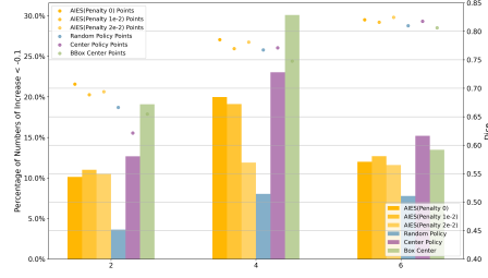
Fig. 3: Misunderstandings and the corresponding performance under different numbers of interactions: The histogram represents the percentage of misunderstanding under different strategies, and the points represent the corresponding dice.
