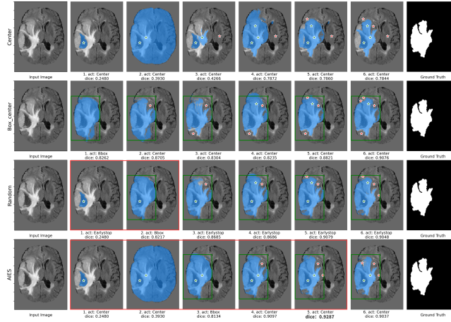
Fig. 4: Visualization of strategies involves Star symbols for center points, green rectangles for bounding box prompts, and red rectangles for actual interaction steps. Subsequent to the red box, counterfactual interactions occur, where interactions continue even though they were actually stopped. In these counterfactuals, the continued interaction specifically uses the "center" form.
