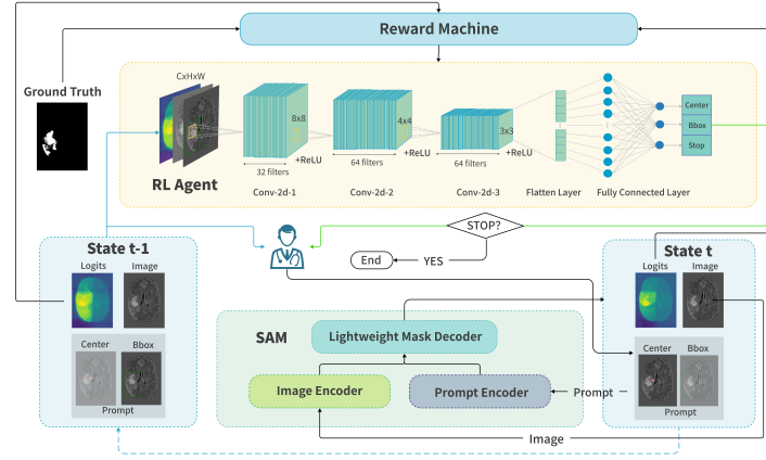
Fig. 1: The architecture of the proposed AIES mechanism: AIES consists of two primary components: the general interactive segmentation model SAM and an RL-based agent. The RL-based agent processes input states, including original medical image slices, previous logits, and prior prompts, subsequently generating recommendations for subsequent interactions within clinical settings. If not terminal, clinicians give SAM new prompts. The medical image slices undergo encoding through SAM’s image encoder, while SAM’s prompt encoder encodes the prompts provided by clinicians. Subsequently, SAM’s lightweight mask decoder generates segmentation logits for the next interaction.
