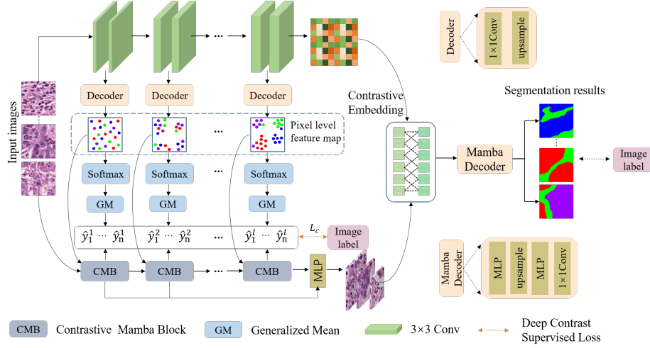
Fig. 1. The overview of the proposed PathMamba. The green block represents the MIML to generate pixel level feature process. Image label is the image-level label.
