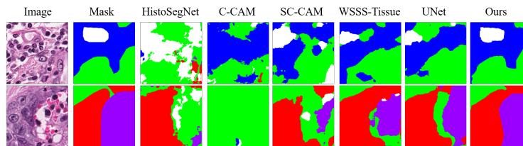
Fig. 3. Visualization of the prediction results of our proposed PathMamba compared with the State of the Art.
