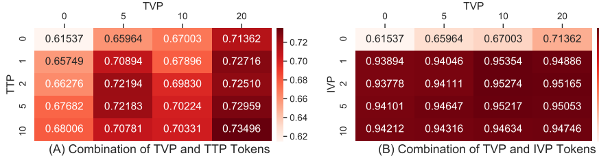
Fig. 4. Comparisons of the PathoTune with different prompt combination.
