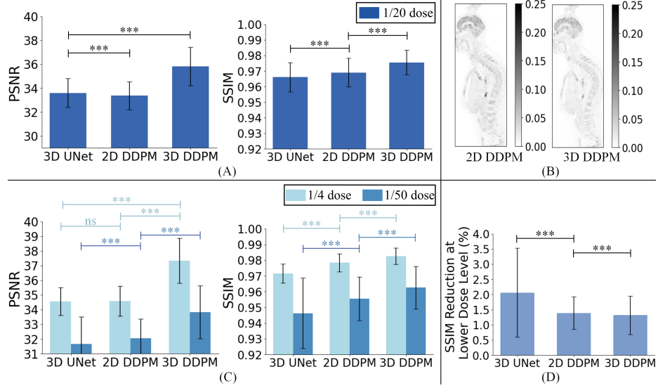
Fig. 4. (A) The PSNR and SSIM values calculated based on 60 1/20 low-dose test datasets. (B) Sagittal view of the uncertainty maps of one test data calculated from 20 realizations for 2D DDPM and 3D DDPM. (C) The PSNR and SSIM values calculated based on 60 1/4 and 1/50 low-dose test datasets, respectively. (D) The SSIM percentage reduction when the dose level of 60 test datasets decreased from 1/20 to 1/50. ***, ns located at the top of the bar plot represents p -value < 0.001 , p -value > 0.05 , respectively.
