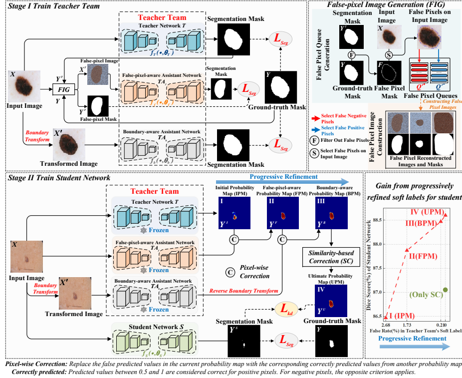
Fig. 1. The overall architecture of PLC-KD.
