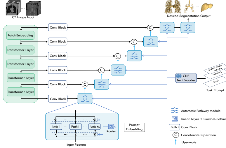
Fig. 1. The overall structure of our model. The decoder encompasses multiple layers with automatic pathway (AP) modules using task-specific prompts as input.
