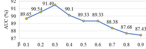
Fig. 3. Performance changes by varying the selection ratio \beta on TCGA MSI dataset.
