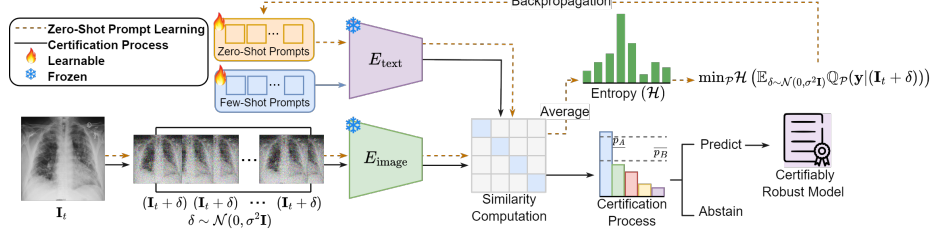
Fig. 1: Overview of PromptSmooth for certified robustness. Prompts can be learned offline or at test-time . Gaussian noise is added at test-time to T copies of the input I_t and prompts are learned by minimizing the entropy loss (dashed orange line). Using zero-shot and/or few-shot prompts, inference is repeated for M noisy instances for certification (solid black line). Model predicts (and gives a certified radius) or abstains.
