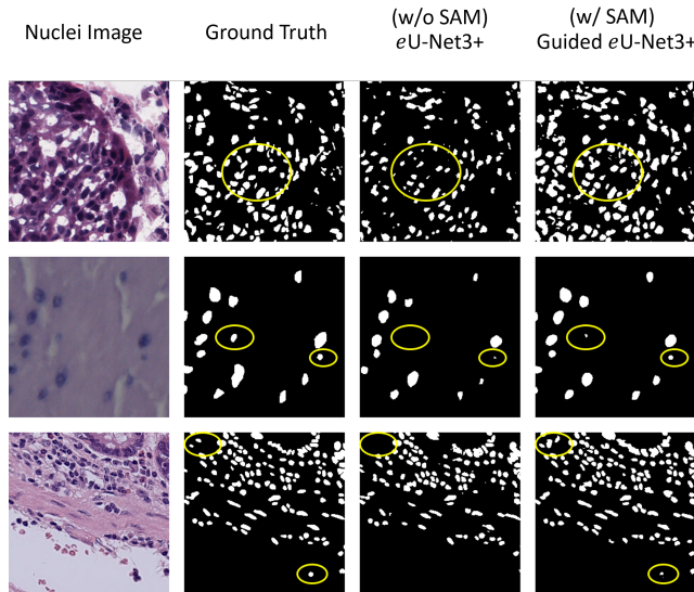
Fig. 4. Qualitative evaluation of segmentation performance of sample images for with and without SAM-guidance for eU-Net3+ . The image in the top row is from CryoNuSeg, middle row is from NuInsSeg and bottom row is from CoNIC.
