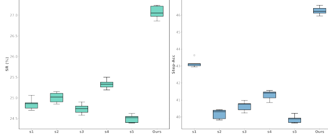
Fig. 3. Boxplot of ablation results with different scales. ‘s1’ to ‘s5’ refer to predefined image scales.
