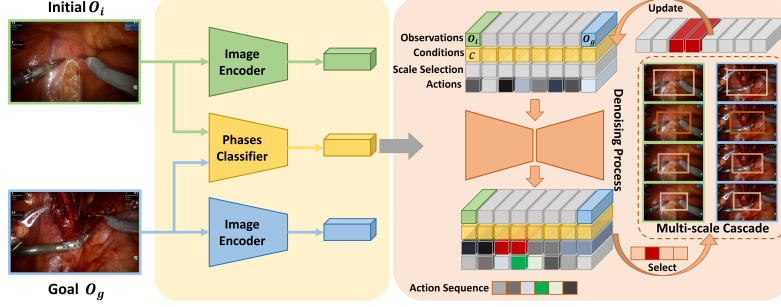
Fig. 1. Overview of our proposed framework. We first generate conditional phase information c by employing a phase classifier, in conjunction with the visual features of initial observations o_i and goal observations o_g for guiding the diffusion process. In the denoising process, we generate multiple scales of inputs and cascade multiple diffusion models that adaptively extract fine-grained visual features for improved performance.
