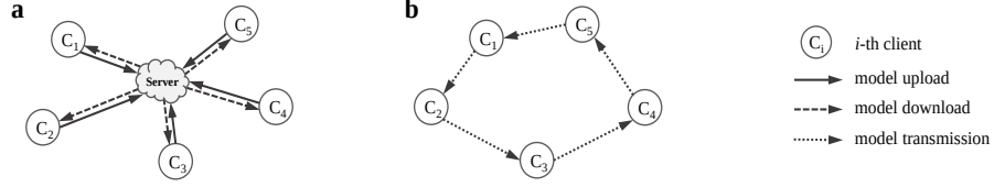
Fig. 1: Comparison between (a) conventional federated learning framework and (b) the proposed serial framework SiFT.
